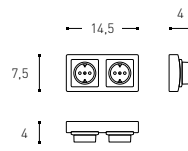
INCH 5.7x1.6x2.9
