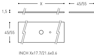
● CRISPLANT COUNTER TOP WITH UPSTAND ENCIMERA CON COPETE CRISPLANT
