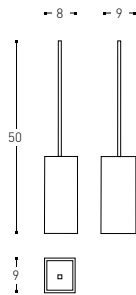
FREE-STANDING OR WALL TOILET BRUSH ESCOBILLERO SUELO/PARED
