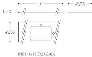
● CRISTALPLANT COUNTER TOP WITH UPSTAND ENCIMERA CON COPETE CRISTALPLANT
