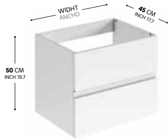
■ □ 2 DRAWERS ADDITIONAL UNIT MUEBLE AUXILIAR CON 2 CAJONES
