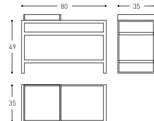
INCH 31.5x13.8x19.3
