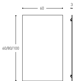
INCH 23.6x23.6/31.5/39.4
