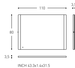
WITH HEATING FOIL FOR MIRROR CON PLACA ANTIVAHO
