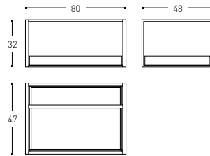
INCH 31.5x18.9x12.6
