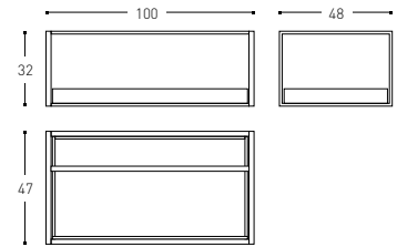
INCH 39.4x18.9x12.6
