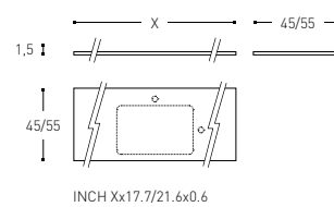
● PHENOLIC RESIN COUNTER TOP WITH UPSTAND ENCIMERA CON COPETE RESINA FENÓLICA
